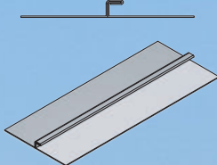
Single Standing Seam Closing
