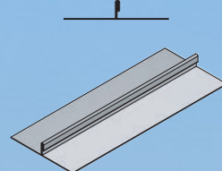
Double Standing Seam Closing
