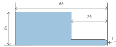
ROUND RAIL 66/24 R = 1.5 - 12
